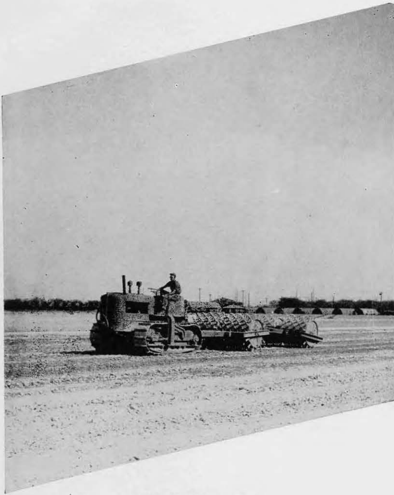
SHEEPSFOOT ROLLER
