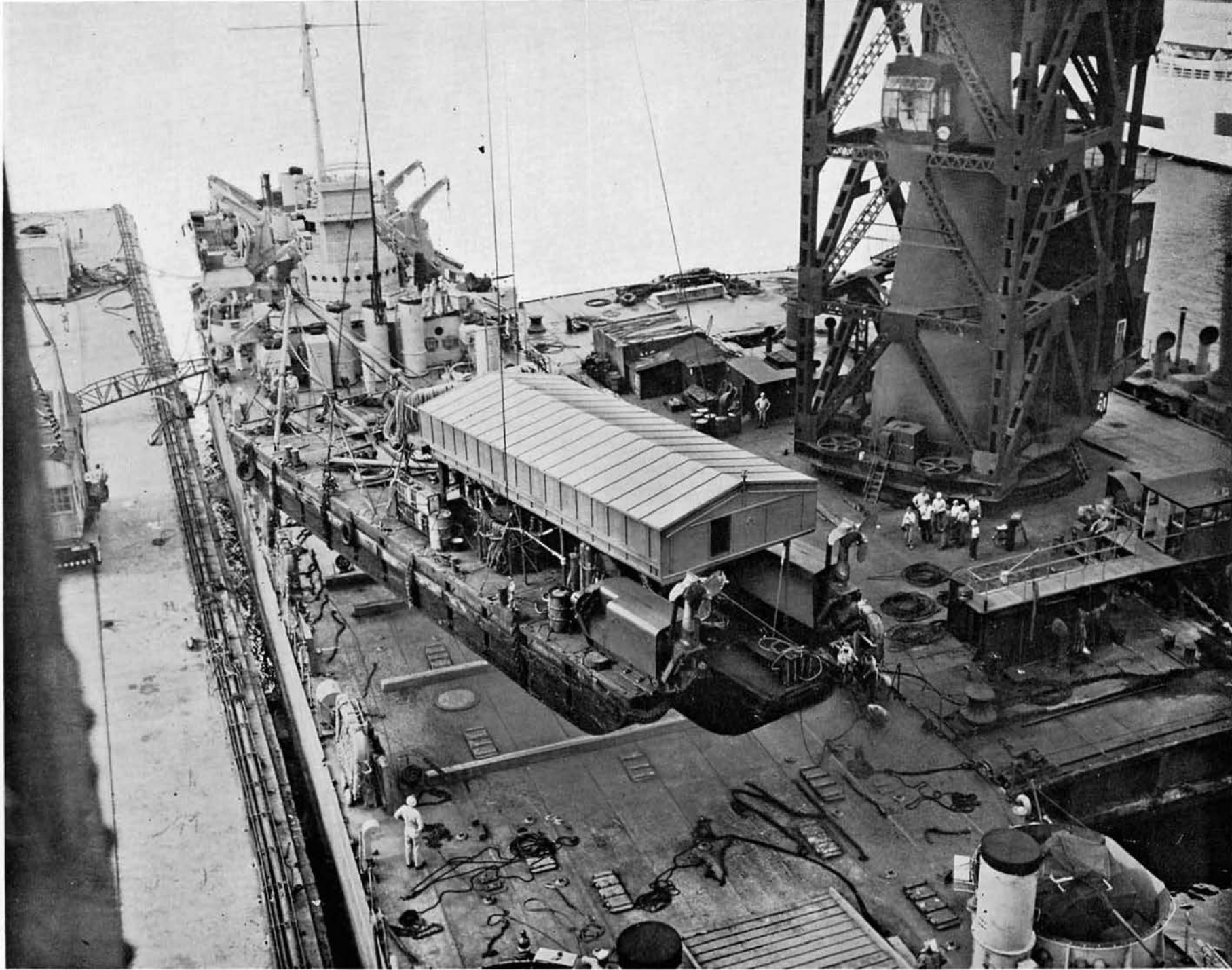
Warping Tug loaded on the deck of an LST in Yokosuka Harbor.
