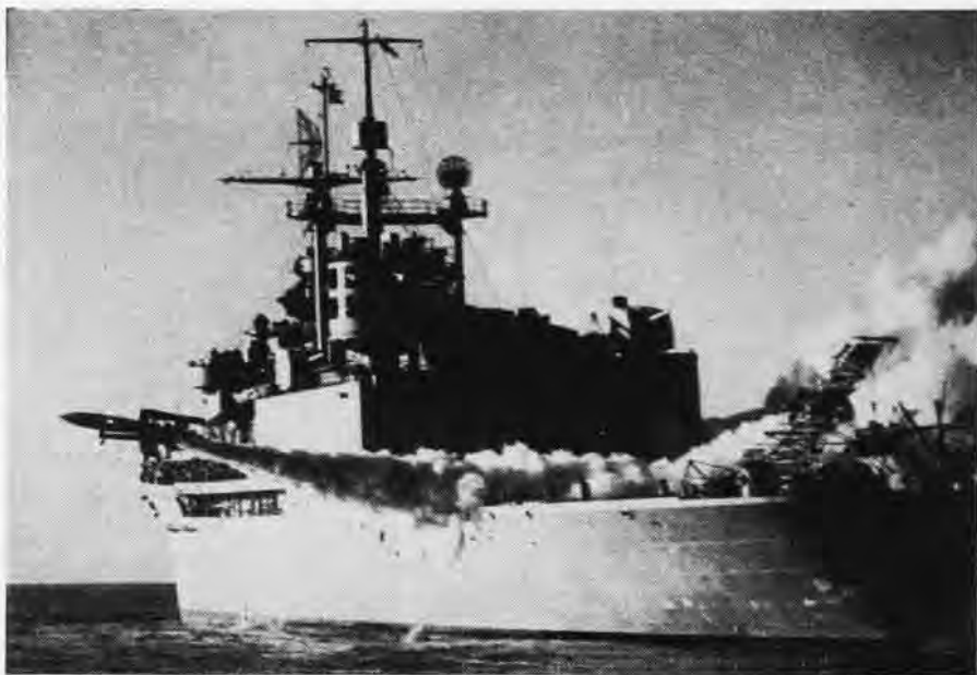
Zooming over the side of the Navy's new experimental guided missile ship the converted seaplane tender Norton Sound is a Loon, American version of the V-1 bomb. A rocket assist unit gives the Loon its initial impetus before its pulsejet motor takes over. Later, the Navy launched the first of a series of Aerobee rockets to measure cosmic rays and terrestrial magnetic fields at high altitudes at the equator.
