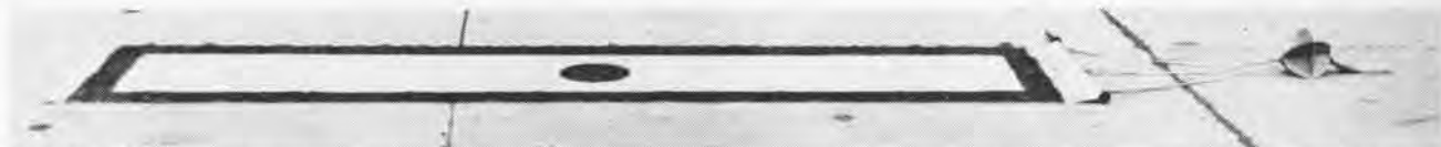
TARGET BANNER , 6'x30' Aero 26B polyethylene, radar-reflective type was towed to supersonic indicated Mach numbers in NATC tests. Ability to withstand high speeds is governed by its limiting Reynold's number. Nylon types had similar durability.
