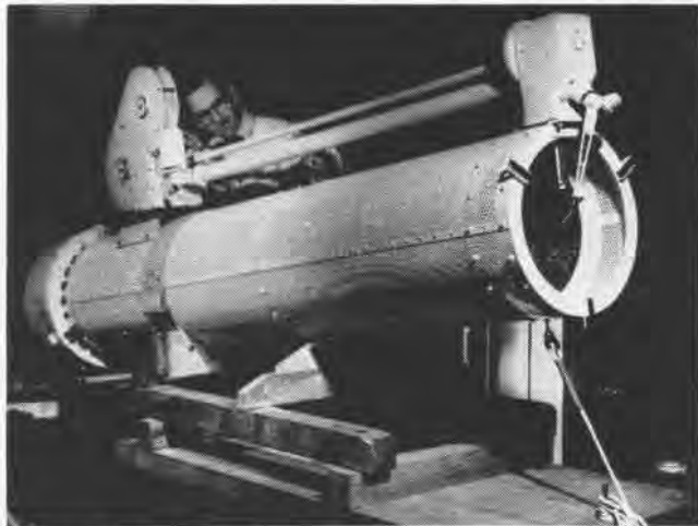
BARREL OF 12-INCH telescope is 9.5 feet long. Here an engineer checks the installation of camera on the outside of the telescope.
