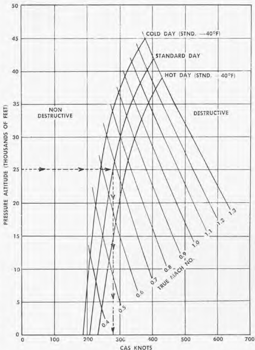
REYNOLD'S NUMBER limitation on Aero 26B banner performance is shown in graph. Example, standard day tow speed limit is less than 280 knots, CAS, .68 true Mach at 25,000 feet.
