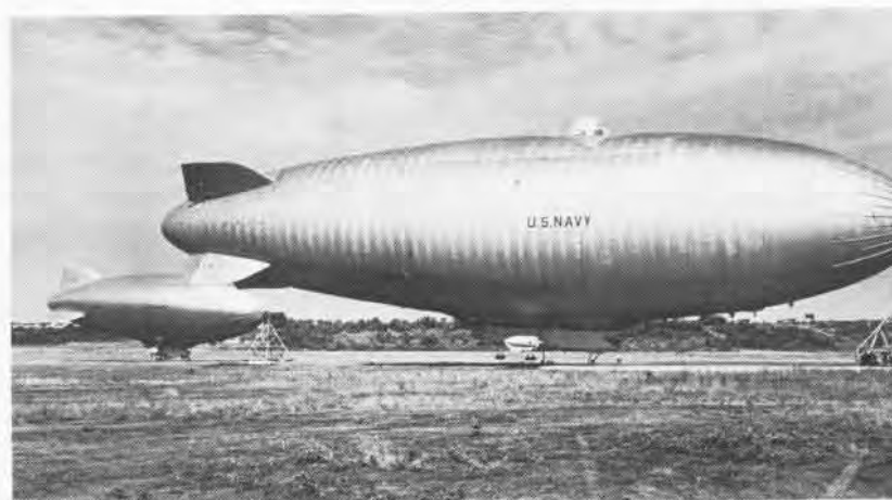
Final Navy non-rigids were 1.5-million-cu.-ft. ZPG-3Ws, AEW airships of the late Fifties.
