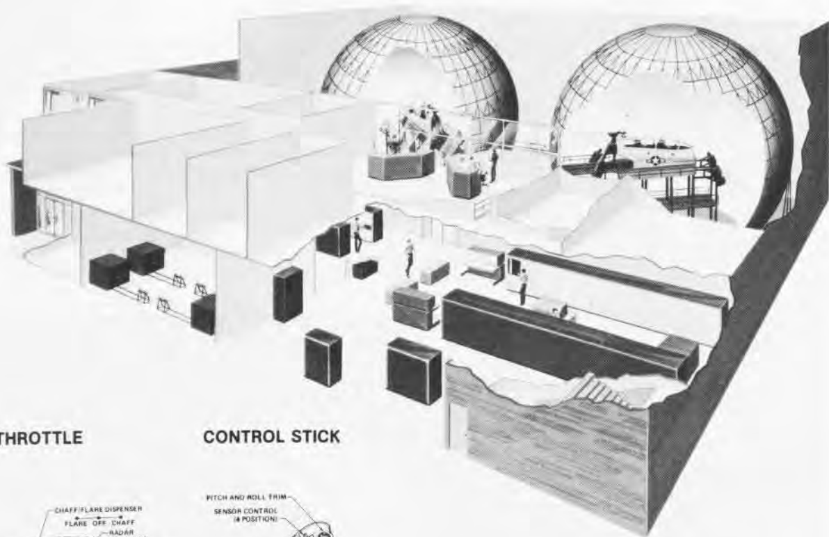
Above, cutaway view of the weapons tactics trainer. Left, schematic views of stick and throttle showing HOTAS functions incorporated into the part task trainer. Below, F/A-18 cockpit showing cathode ray tubes with alphanumeric displays.
